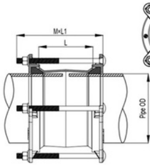
SLEEVE TYPE COUPLING
